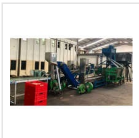
Mild Steel Cashew Cutting Machine
